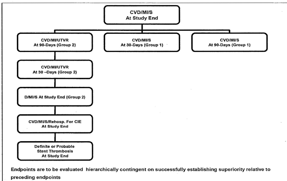
Figure 4: Hierarchical plan for secondary endpoints
