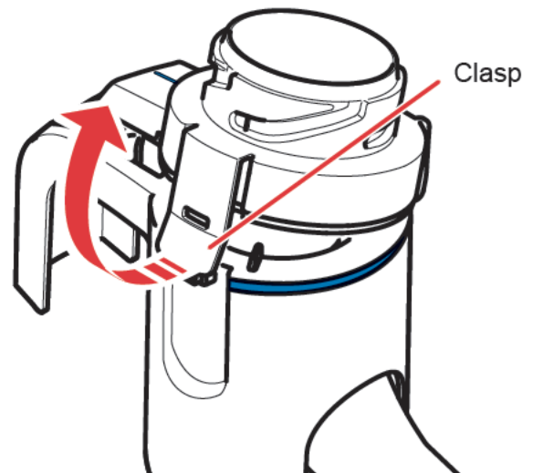
Fig. D2 Open the Handset body.
