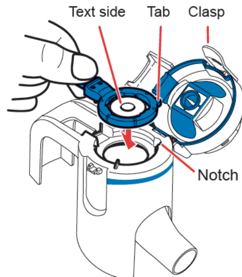
Fig. D3 Insert the Aerosol head into the Handset body. Do not touch the center of the Aerosol head.
