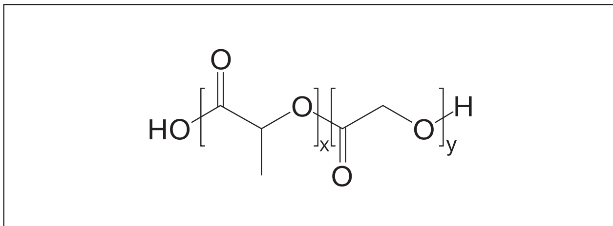
Figure 2.2 The Chemical Structure of PLGA
