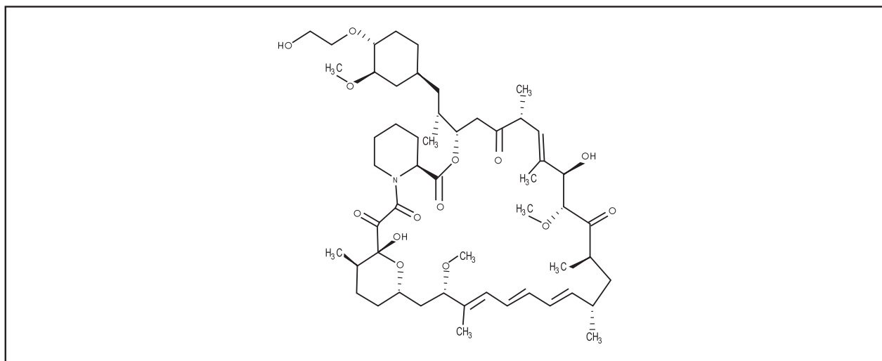
Figure 2.1 The Chemical Structure of Everolimus
