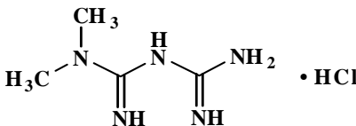
Metformin Hydrochloride
