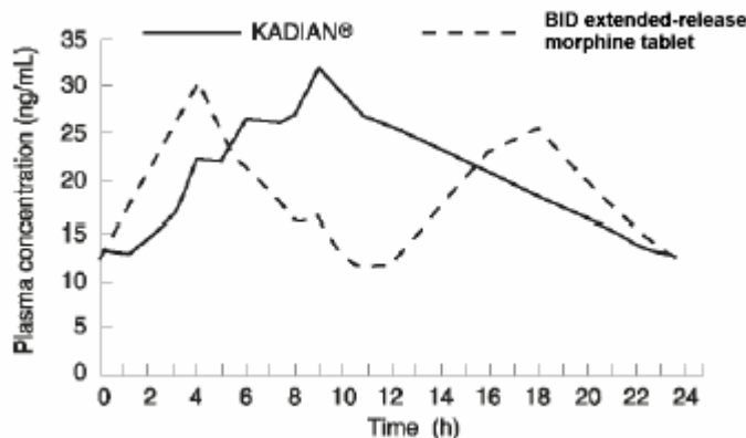
Graph 2 (Study # MOR-9/92): Dose normalized mean steady state plasma morphine concentrations for KADIAN® (once a day), and an equivalent dose of a 12-hour, extended-release morphine tablet given twice a day. Plasma concentrations are normalized to 100 mg every 24 hours, (n=24).
