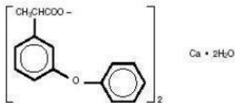
Benzenaetic acid, \alpha -methyl-3-phenoxy-, calcium salt dihydrate, ( \pm )
