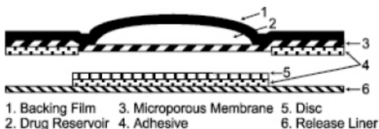
Figure 1: System Schematic
