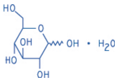
D-Glucose monohydrate
