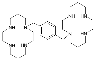
Figure 1: Structural Formula
