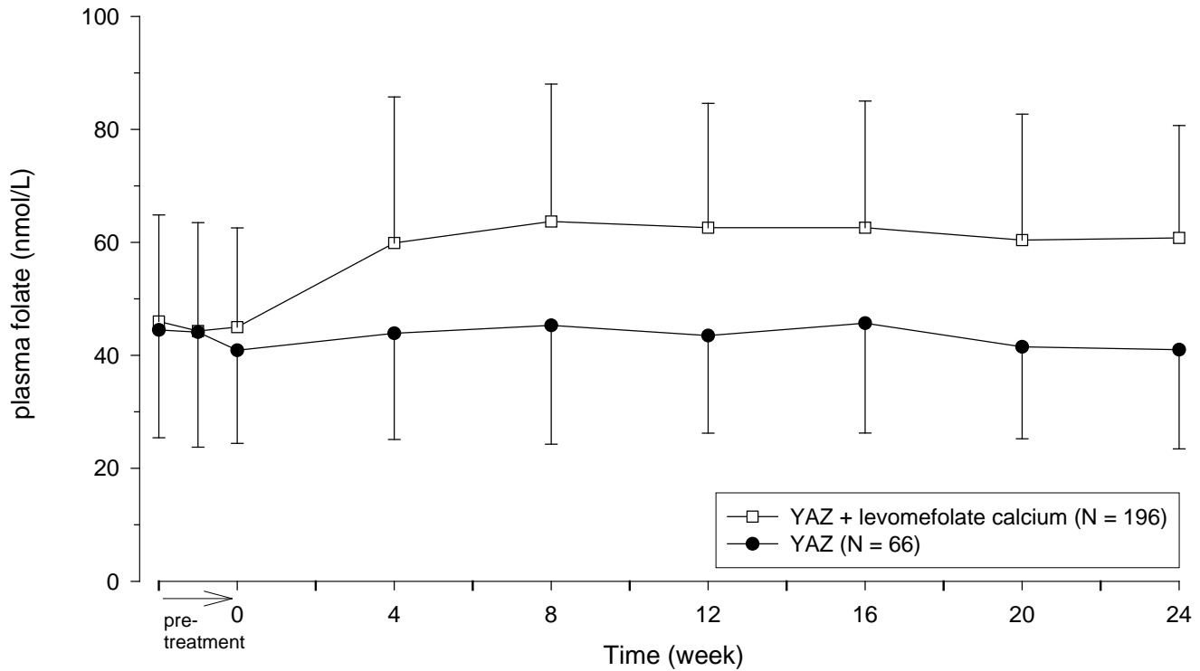
Figure 3: US Study: Mean concentration-time curves (and SD) of plasma folates after daily oral administration of YAZ + levomefolate calcium and YAZ
