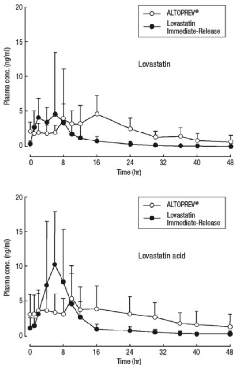
Figure 1 Mean (SD) plasma concentration-time profiles of lovastatin and lovastatin acid in hypercholesterolemic patients (n=12) after 28 days of administration of Altprev® or lovastatin immediate-release
