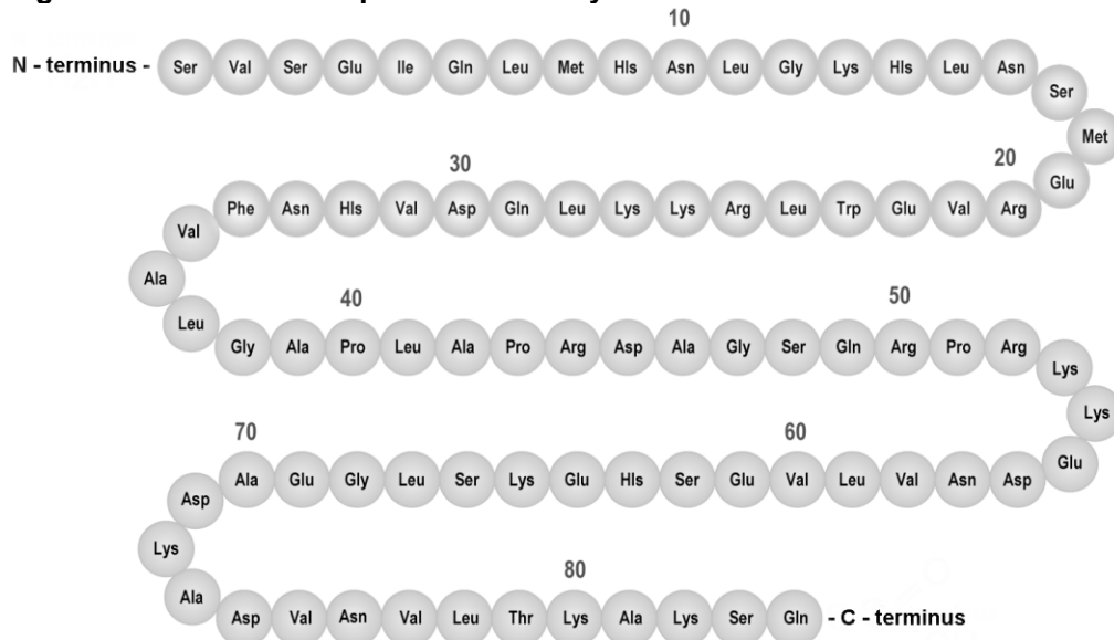
Figure 1: Amino Acid Sequence of Parathyroid Hormone
