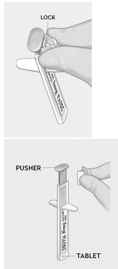
Figure 2. Lock Removal
