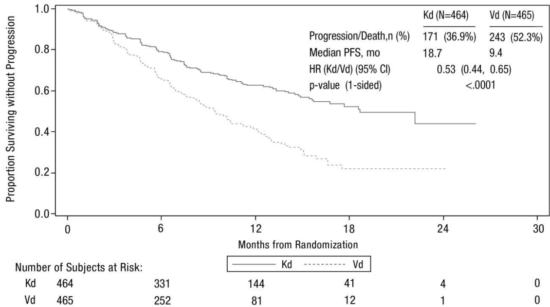
Figure 3: Kaplan-Meier Plot of Progression-Free Survival in ENDEAVOR
