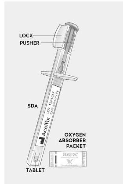
Figure 2. Lock Removal
