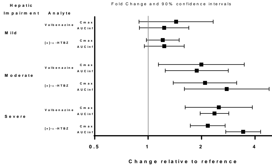
Figure 1: Effects of Hepatic Impairment on Valbenzine Pharmacokinetics
