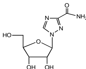
Figure 1: Structural Formula
