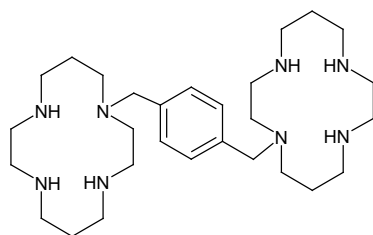
Figure 1: Structural Formula
