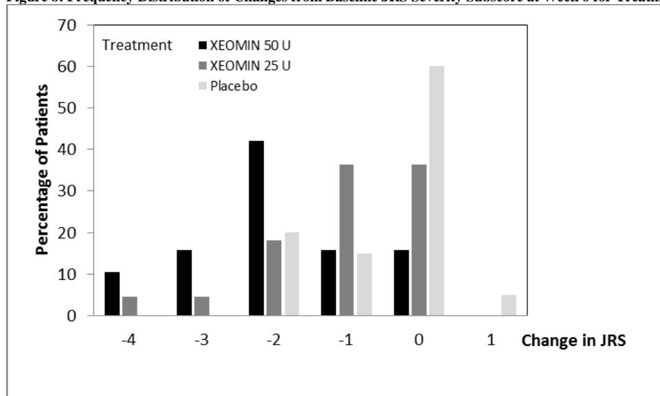
Figure 8: Frequency Distribution of Changes from Baseline JRS Severity Subscore at Week 6 for Treatment-Naive Patients
