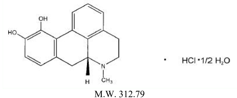
Figure 1: Structural Formula and Molecular Weight of Apomorphine
