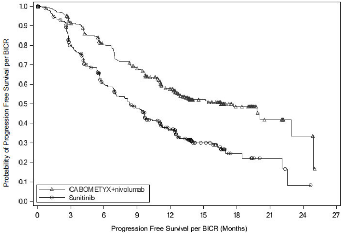
Figure 5: Kaplan-Meier Curve of Progression-Free Survival in CHECKMATE-9ER
