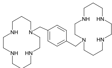
Figure 1: Structural Formula
