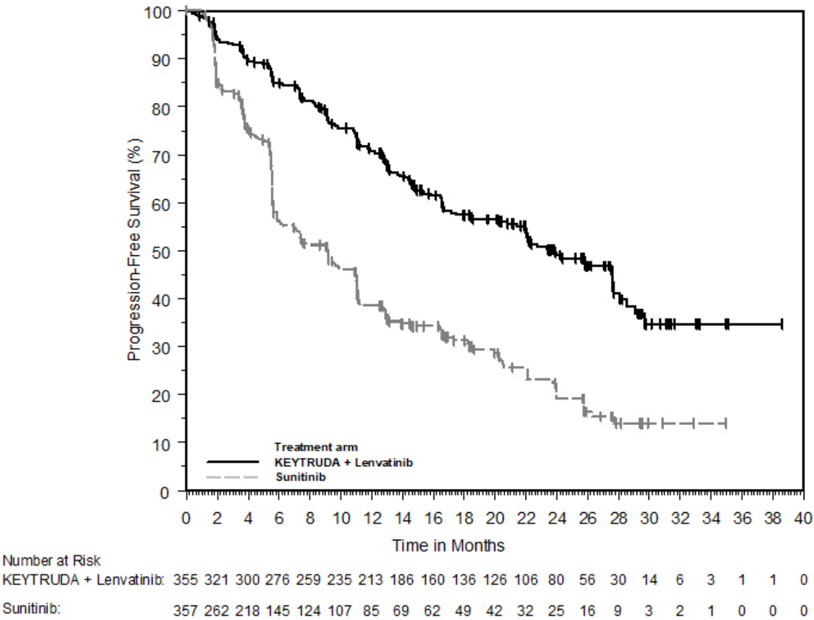
Figure 20: Kaplan-Meier Curve for PFS in KEYNOTE-581
