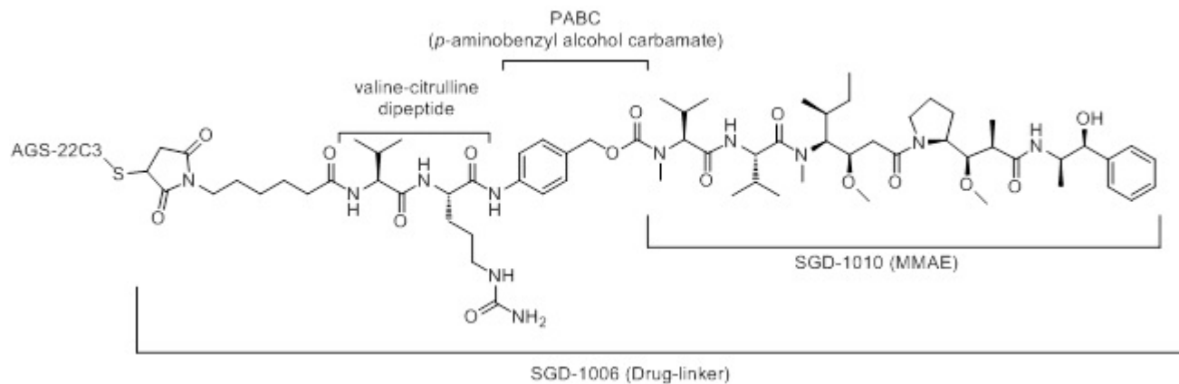
Figure 1. Structural Formula
