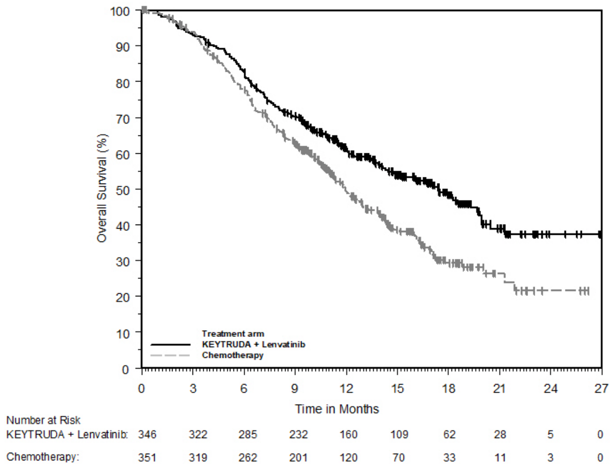
Figure 31: Kaplan-Meier Curve for Overall Survival in KEYNOTE-775 (pMMR or Not MSI-H)
