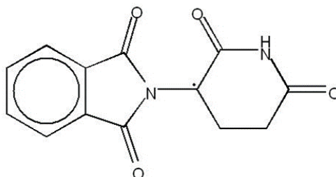
Chemical Structure of Thalidomide
