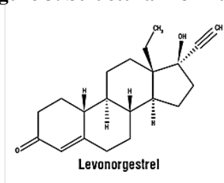
Figure 3. Structural Formulas
