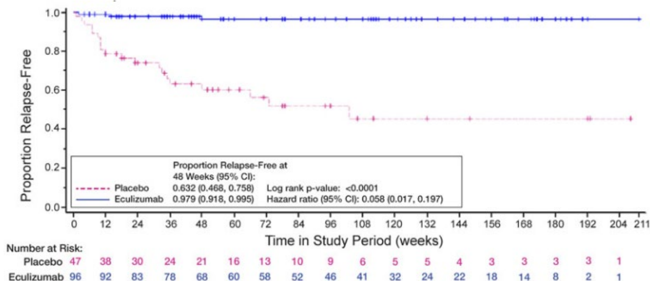
Figure 1: Kaplan-Meier Survival Estimates for Time to First Adjudicated On-Trial Relapse – Full Analysis Set
