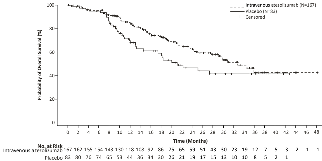
Figure 12: Kaplan-Meier Plot of Overall Survival in IMvigor011
