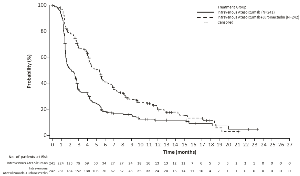
Figure 8: Kaplan-Meier Plot of Overall Survival in IMforte
