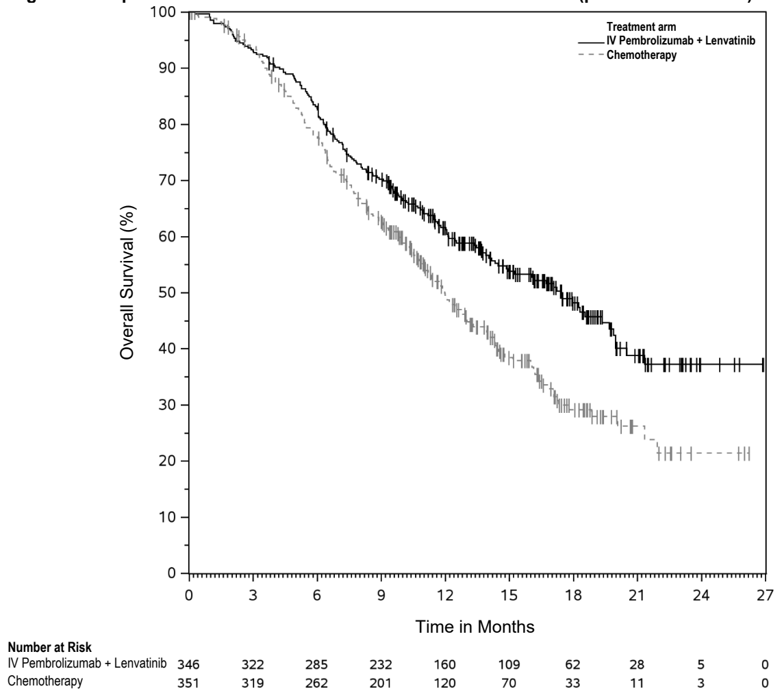
Figure 40: Kaplan-Meier Curve for Overall Survival in KEYNOTE-775 (pMMR or Not MSI-H)
