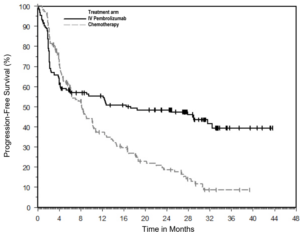
Figure 21: Kaplan-Meier Curve for PFS in KEYNOTE-177
