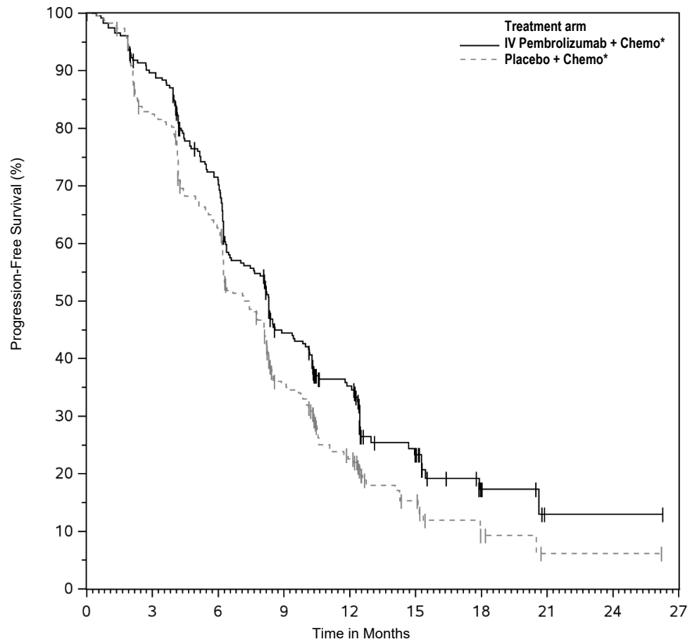
Figure 46: Kaplan-Meier Curve for Progression-Free Survival in KEYNOTE-B96 (CPS \geq 1 )
