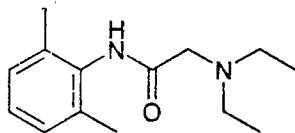
Lidocaine C_{14}H_{22}N_2O M.W. 234.3
