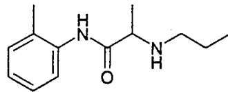
Prilocaine C_{13}H_{20}N_2O M.W. 220.3
