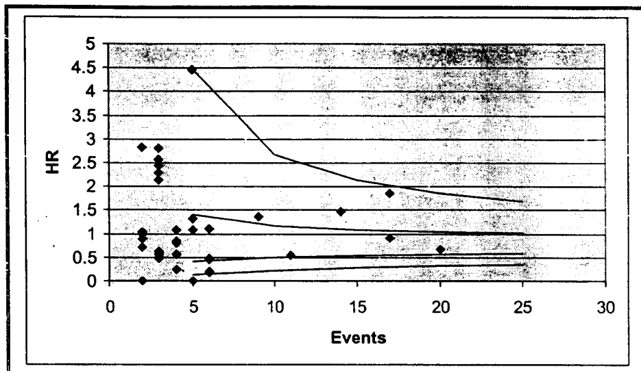
Figure 6. Hazard ratio for mortality by center (CAPRICORN)
