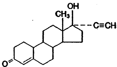
NORETHINDRONE
