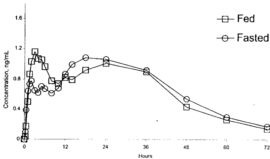
FIGURE 2. Single-Dose Palladone™ Pharmacokinetic Profiles
