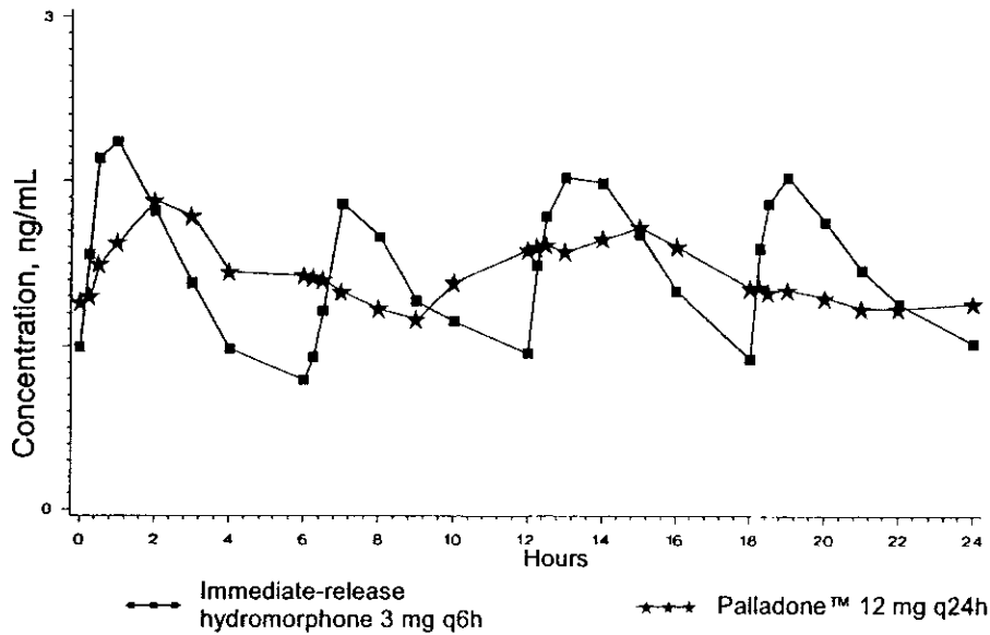
FIGURE 1. Steady-State Plasma Hydromorphone Concentration-Time Curves
