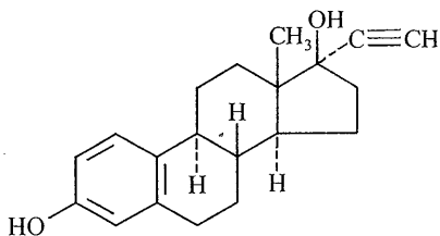
Ethinyl Estradiol [19-Norpregna-1,3,5(10)-trien-20-yne-3,17-diol, (17 \alpha )-]
