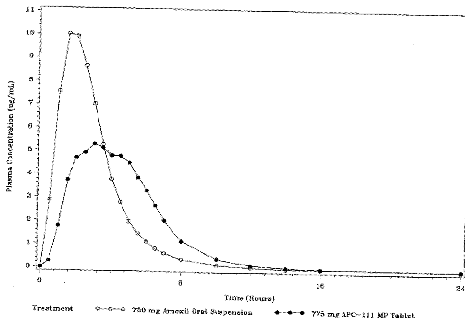
Figure 1.3-1 Mean Total Plasma Amoxicillin Concentration vs. Time Curves for Single Doses of 750 mg Amoxicillin Suspension and 775 mg APC-111.
