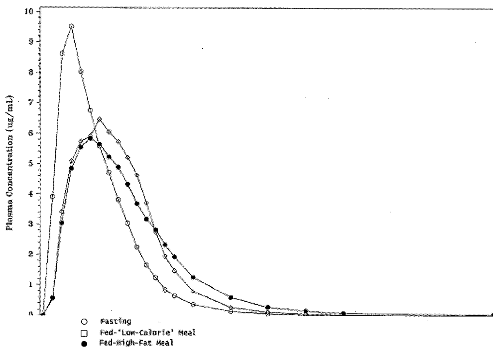
Figure 1. Mean Plasma Amoxicillin Concentration vs. Time Curves for APC-111 Under Fasting, Low-Calorie Fed and High-Fat Fed Conditions.
