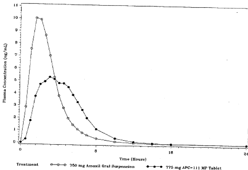
Figure 1. Mean Plasma Amoxicillin Concentration vs. Time Curves for Single Doses of 750 mg Amoxil® Oral Suspension and 775 mg APC-111
