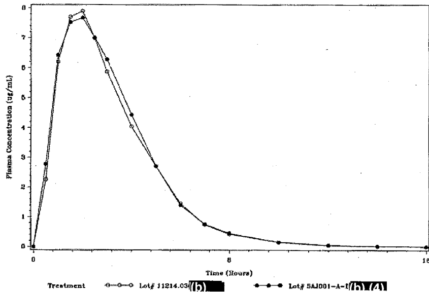
Figure 1. Mean (Total) Plasma Amoxicillin Concentration vs. Time Plots
