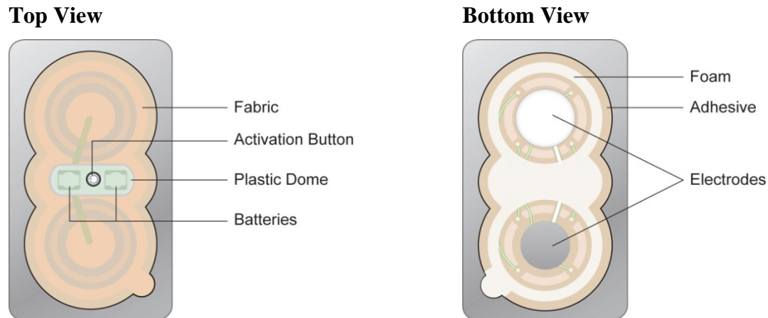
Figure 2: Iontophoretic Device
