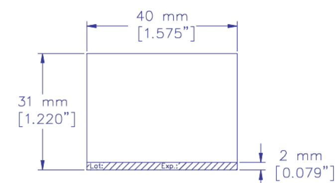
INDIVIDUAL BLISTER CELL
