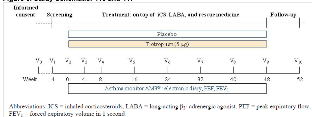
Figure 6. Study Schematic: 416 and 417
