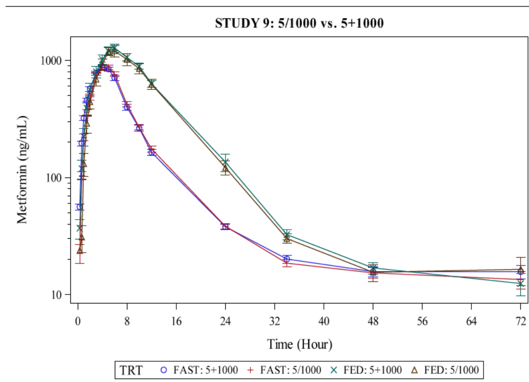
Figure 3 Mean (SE) linagliptin (left) or metformin (right) concentration – time profiles by treatments
