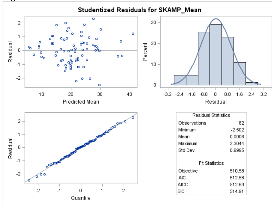
Figure 3. Studentized Residuals for SKAMP-Combined Mean Scores
