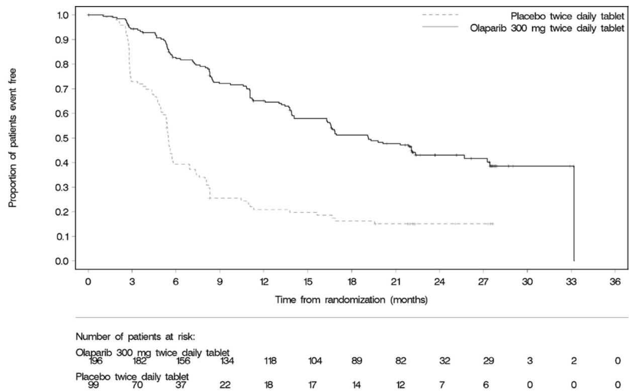
Figure 1: Kaplan-Meier Curves of Investigator-Assessed Progression-Free Survival – SOLO-2
