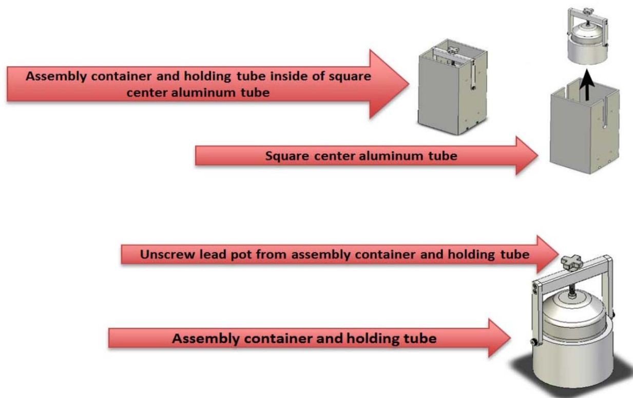
Figure 2: Unpacking for lead pot containing AZEDRA
