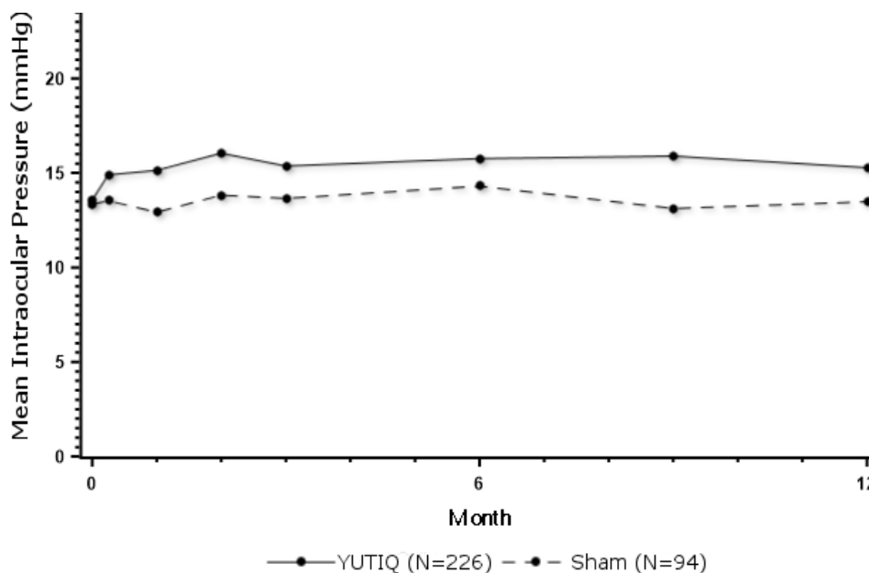
Figure 1: Mean IOP During the Studies
