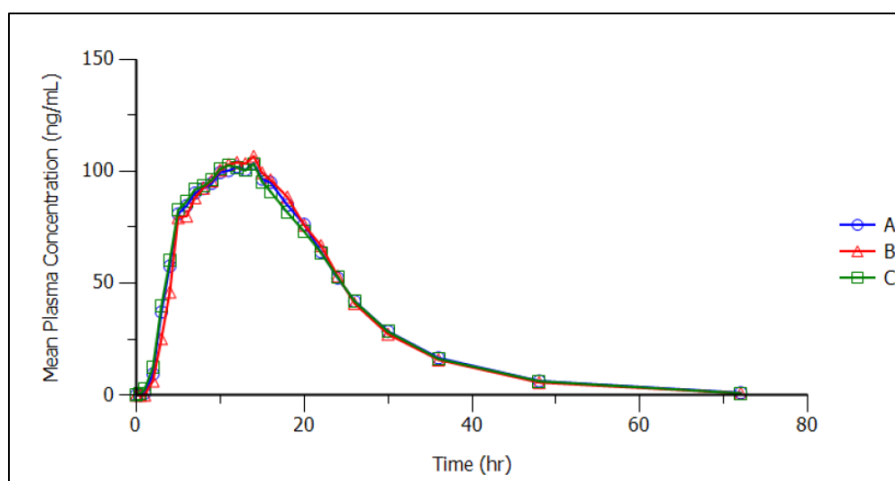
Figure 1. Linear scale plot of mean plasma concentration vs time profiles of metoprolol – by treatment
