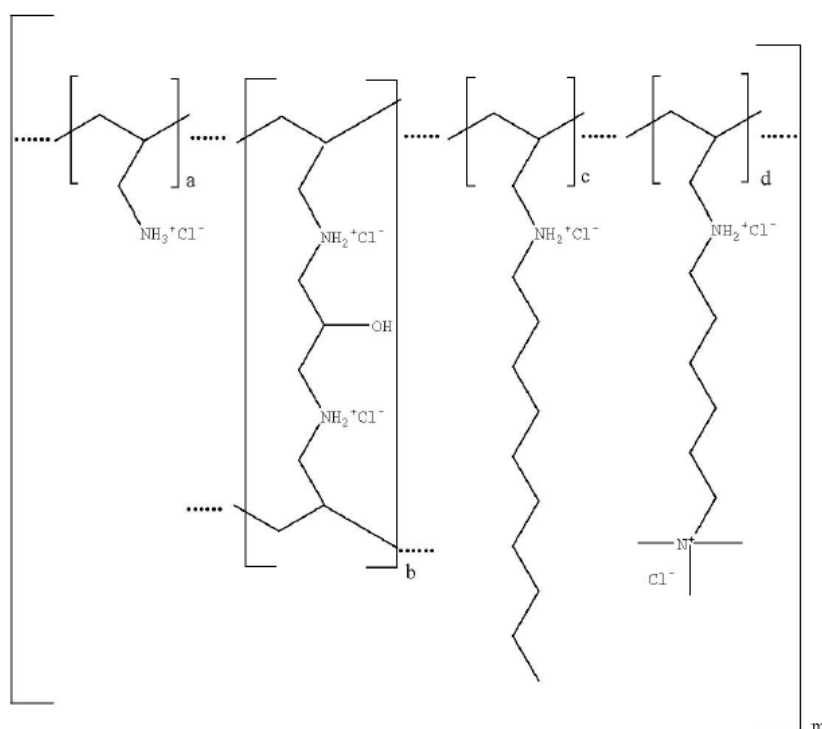
Figure 1: Chemical structure of colesevelam HCl where in (a) represents allyl amine monomer units that have not been alkylated by either of the 1-bromodecane or (6-bromohexyl)-trimethylammonium bromide alkylating agents or cross-linked by epichlorohydrin; (b) represents allyl amine units that have undergone cross-linking with epichlorohydrin; (c) represents allyl amine units that have been alkylated with a decyl group; (d) represents allyl amine units that have been alkylated with a (6-trimethylammonium) hexyl group, and m represents a number \geq 100 to indicate an extended polymer network. A small amount of the amines is dialkylated, and are not depicted in the formula above.
