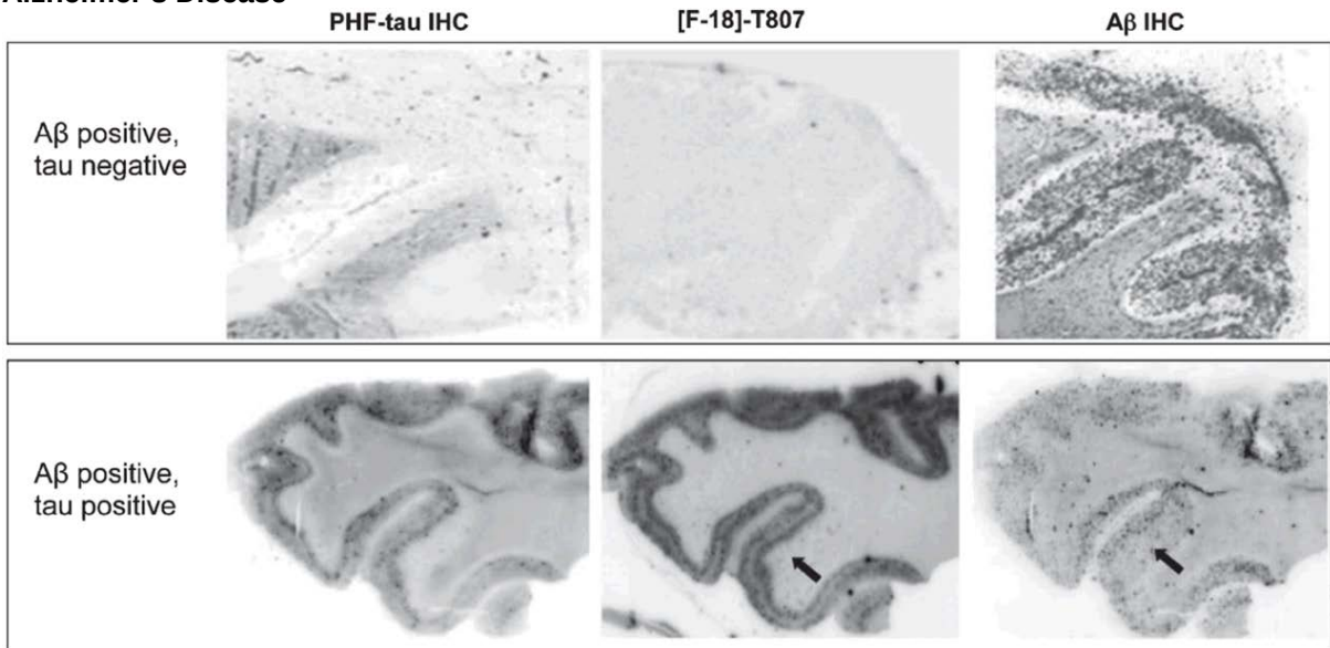
Figure 3. FTP Autoradiography and Immunohistochemistry of Brain Sections from Patients with Alzheimer's Disease
