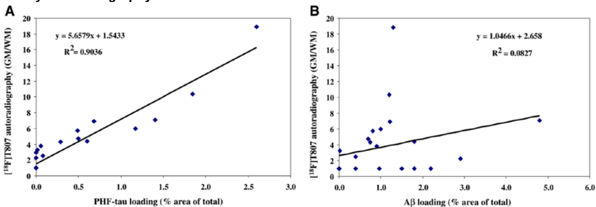
Figure 4. Correlations of FTP ( 18 F-T807) Binding With PHF-Tau (A) and β-Amyloid Aggregate (B) IHC by Autoradiography
