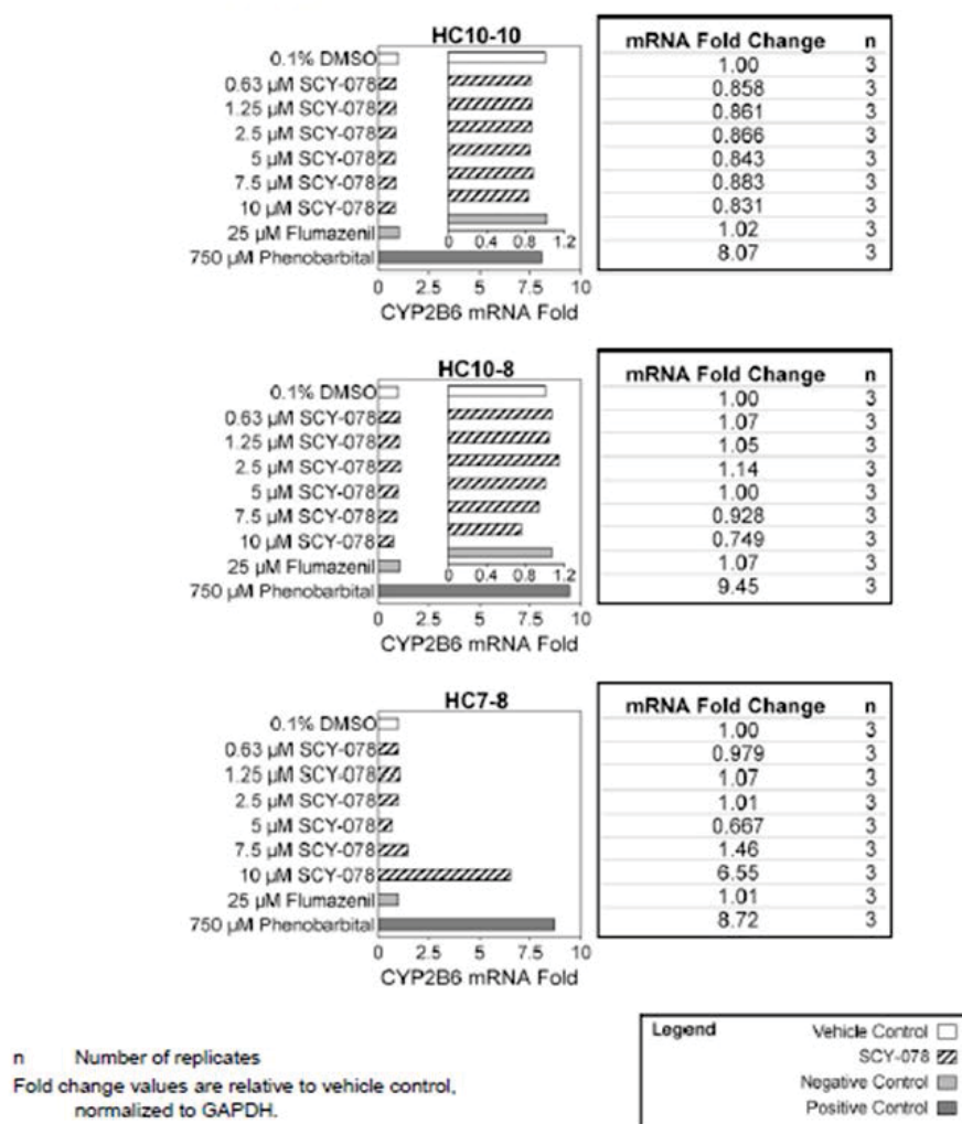
Figure 6. CYP3A4 fold change: The effect of treating cultured human hepatocytes with ibrexafungerp on CYP3A4 mRNA levels
