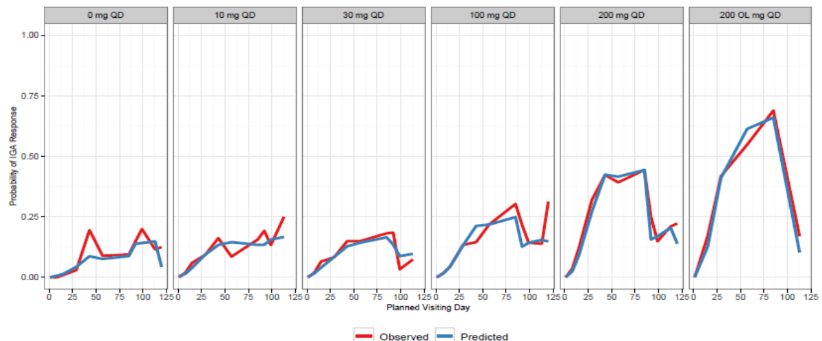
Figure 31. Predicted Probabilities of Responding Over Time by Dose Group for the Final IGA Model
