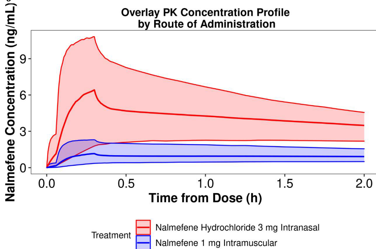
Figure 25: PK Simulation of IN and IM Administration
